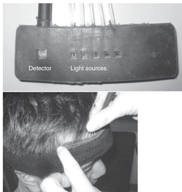
Figure 1. fNIRS sensor with linearly arranged light sources and detector (top). Two such sensors were placed next to each other on the forehead and secured with a headband (bottom) over the Fp1 and Fp2 locations.
