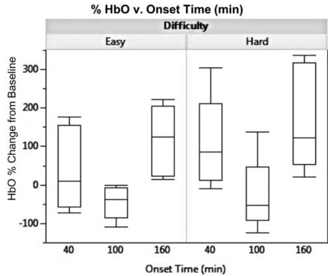
Figure 5. Box plot indicating HbO % change from reference for the six experimental conditions.
